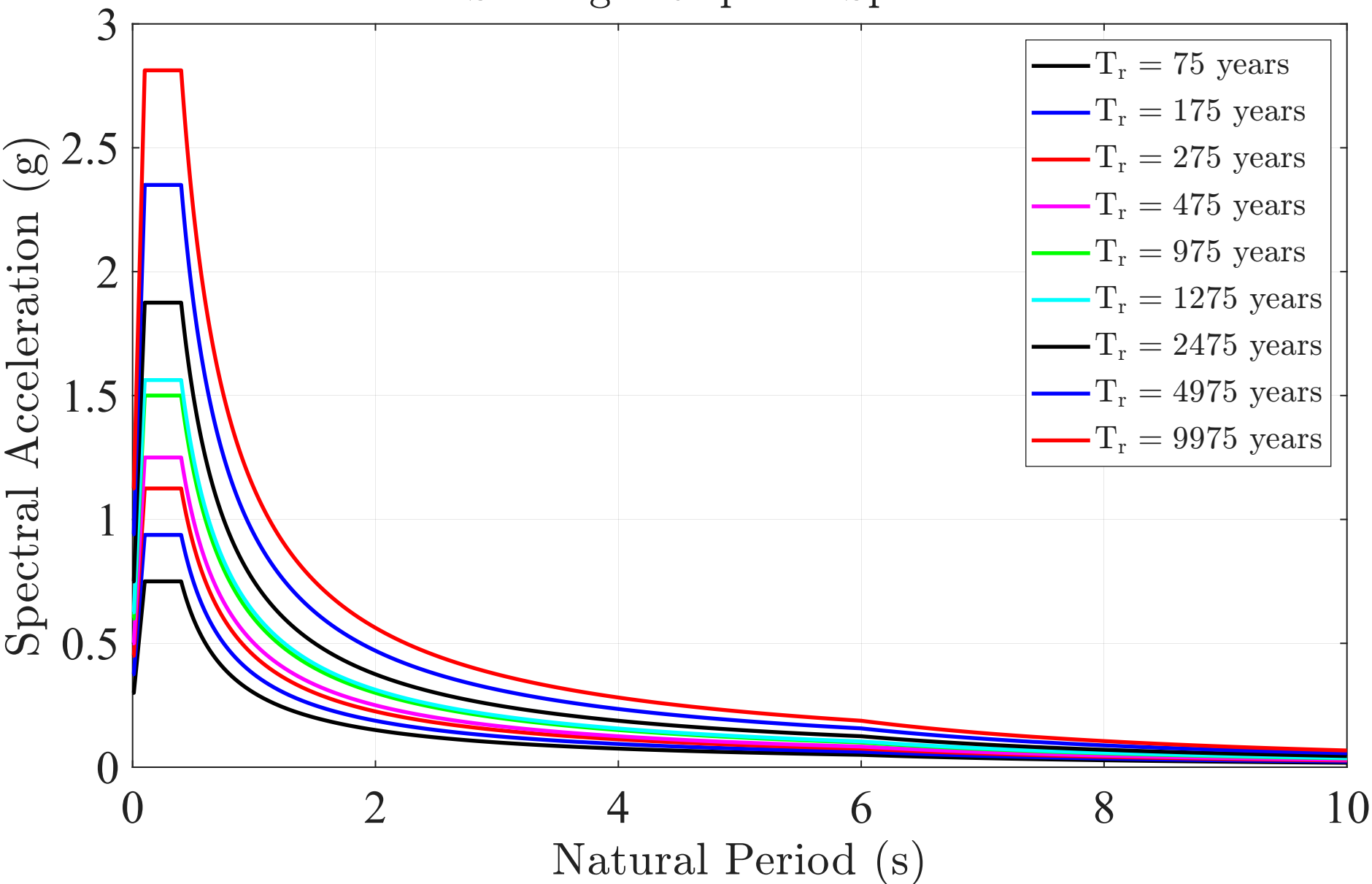
IS Design Response Spectrum
